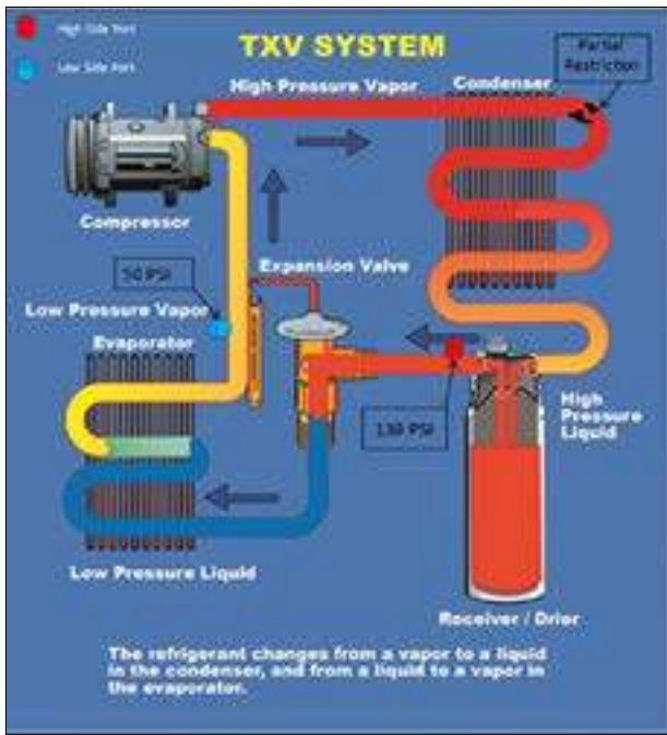
Figure 5: Expansion Valve System with a restricted condenser.
