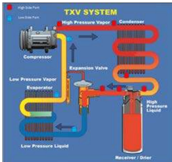
Figure 2: Expansion Valve System Service Port "Wish List".
