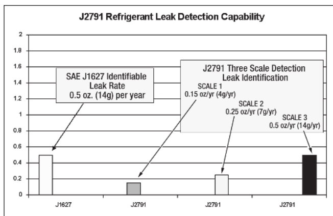
Chart B: This chart compares the effectiveness of SAE J1627 and J2791 electronic leak detectors.
