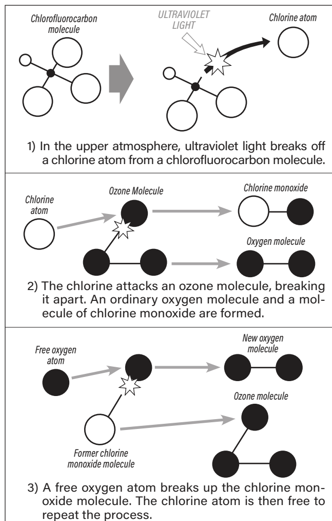
Chlorine atoms from CFCs break apart ozone molecules. This results in a reduction of stratospheric ozone.
